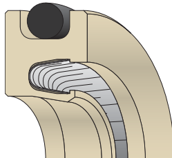
Chamfered ID, O-Ring OD Rotary FlexiSeal
