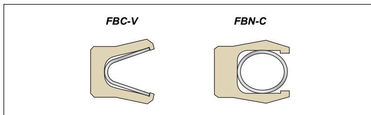
Figure 2-19. Chamfered Lips
