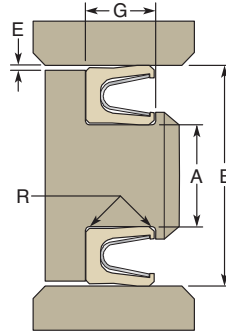
Piston Seal
