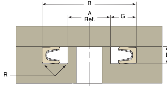
Internal Pressure
