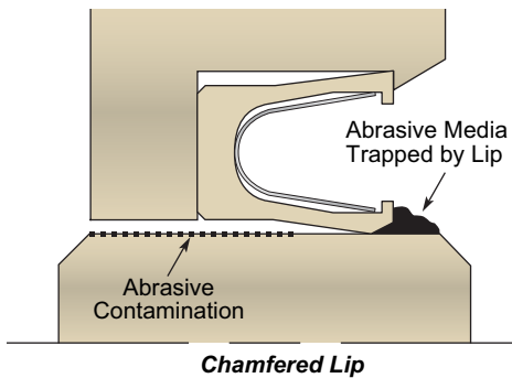
Chamfered Lip
