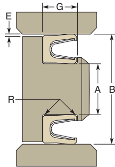
Piston Seal
