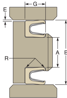
Piston Seal
