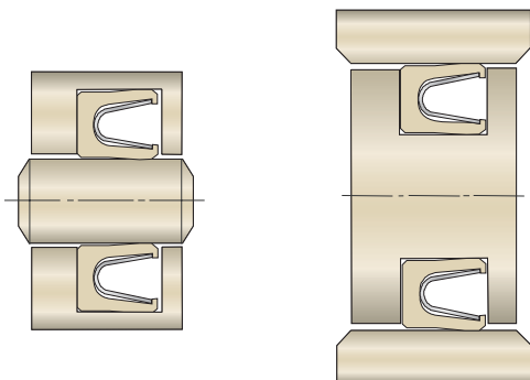
Closed Glands
