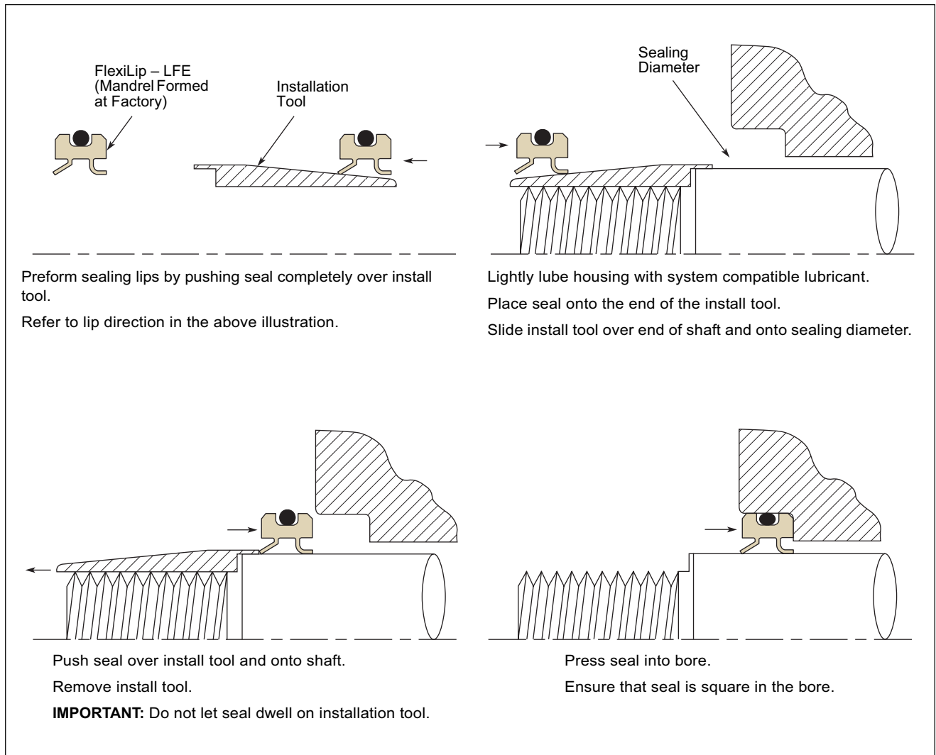
Figure 8-1. FlexiLip Installation
