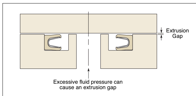
Figure 6-1. Fluid Pressure Causes Extrusion Gap
