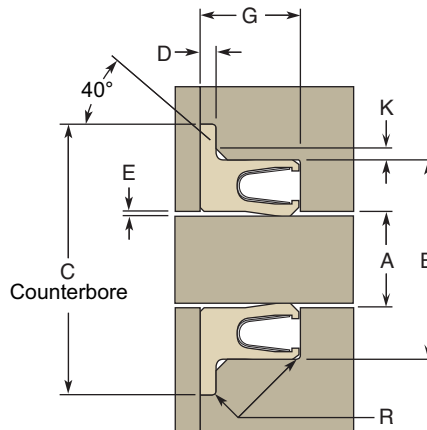
Flanged Seal
