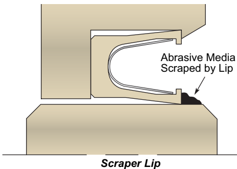
Scraper Lip
