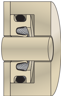
Rotary Application
