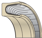
Chamfered Rod/Piston Seal with Cantilever Spring
