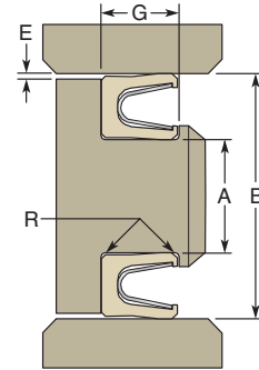
Piston Seal
